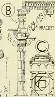
DIAGRAMS OF HINDU TEMPLE CONSTRUCTION AFTER FERGUSSON - FIG C SHOWS SECTION & PLAN LOOKING UP. COLUMNS & LINTELS SUPPORT COURSES OF STONE SABS. FIG B SHOWS METHOD OF STRENGTHENING LINTEL BY BRACKET.
