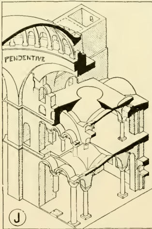
S. SOPHIA CONSTANTINOPLE SECTIONAL VIEW
