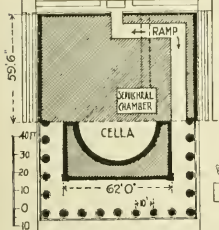
HALF PLAN OF BASEMENT B HALF PLAN OF PERISTYLE
