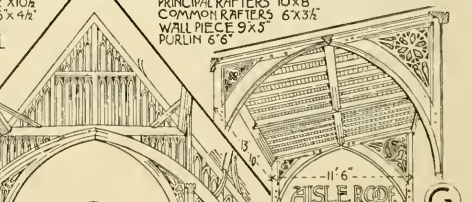
(G) AISLE ROOF. NEW WALSINGHAM
