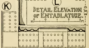
(K) (L) DETAIL ELEVATION OF ENTABLATURE.
