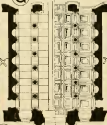
(H) ENLARGED PLAN LOGGIA
