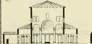
SECTION G
