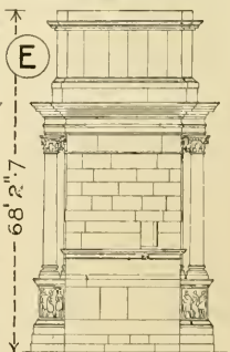
END ELEVATION THIS TRIUMPHAL ARCH WAS DEDICATED BY THE ROMANS IN HONOR OF THE EMPEROR SEPTIMIUS SEVERUS FOR HIS VICTORIES IN THE EAST IN CONJUNCTION WITH HIS 2 SONS CARACALLA & GETA
