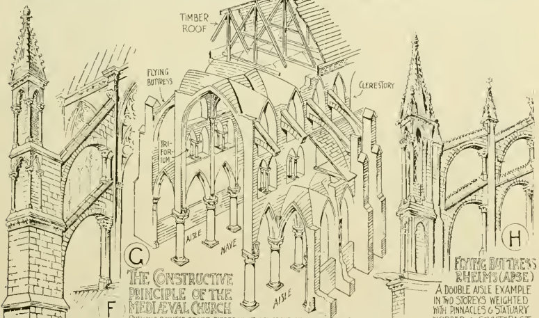
F FLYING BUTTRESS (AMIER'S) ASINGLE AISLE EXAMPLE IN TWO TIERS, WEIGHTED WITH PINNACLE.
