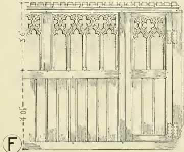
PARCLOSE SCREEN, GEDDINGTON CH., NORTHANTS.
