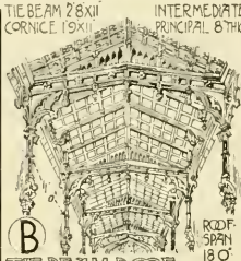
(B) TIE BEAM ROOF. TRINITY CHAPEL, CRENSHAW THIS FORM USED THROUGHOUT MIDDLE AGES
