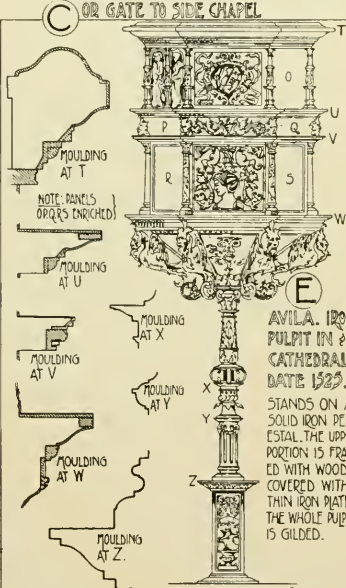
SCALE OF INCHES FOR MOULDINGS 1 2 3 4 5 SCALE OF FEET FOR ELEVATION
