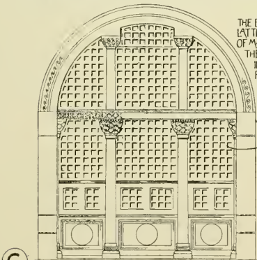
G ELEVATION WINDOW FROM THE GALLERY (GYMNECEUM) S. SOPHIA CONSTANTINOPLE
