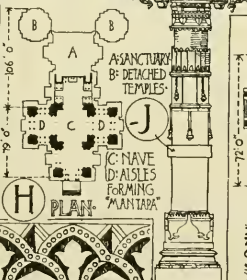
TEMPLE AT BINDRABUND. AGRA AD 1592. INDO-ARYAN. J. C. NAIVE D'AISLES FORMING 'MANTARA'. K. PLAN. L. PLAN.
