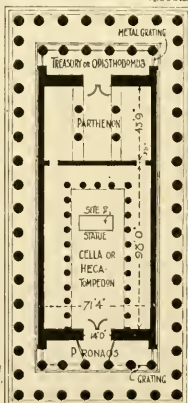
(H) PLAN (AFTER RENOIR)
