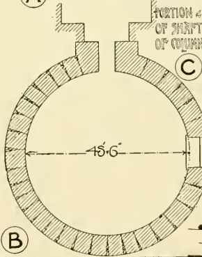
(B) PLAN OF THE TREASURY OF ÆTREUS
