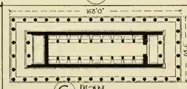
(C) PLAN
