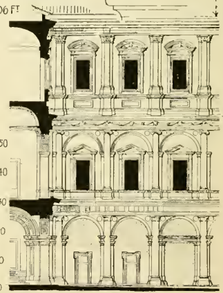
(E) FIRST ELEVATION OF CORTILE
