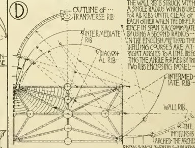
GOthic VAULT WITH WALL BRIDGE RIBS OBLONG COMPARTMENT DIFFERENCE OF SPAN ACCOMMODATED BY USING POINTED ARCHES OF DIFFERENT RADII
