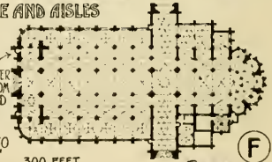
F PLAN
