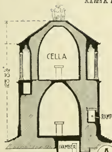
TRANSVERSE SECTION A
