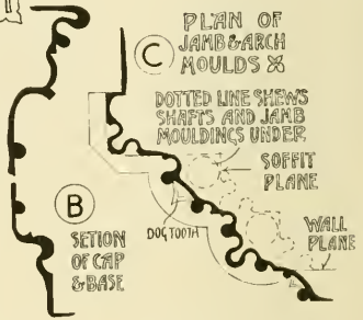
PLAN OF JAMB & ARCH MOULDS
