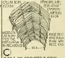
(C) COLLAR BRACED ROOF. ST MARY MAGDALEN, PULHAM, NORFOLK THIS ROOF IS A SIMPLIFICATION OF HAMMER BEAM
