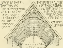
(A) TRUSSED RAFTER ROOF. STOWE BARDOLPH CHURCH, NORFOLK EARLY FORM USED TO OBTAIN HEADWAY
