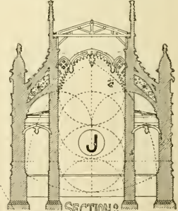
SECTION OF HENRY VII'S CHAPEL
