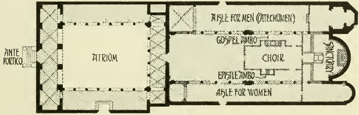
(B) PLAN
