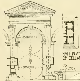
D DOORWAY OR PORTION OF IONIC COLONNADE WITHOUT PEDESTALS.
