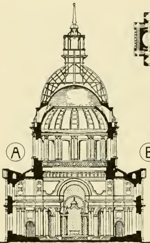
A. A.D. 1670 SECTION THROUGH DOME. JULES MANTO, 1706. THE INVALIDES, PARIS, SARD, ARCHT.
