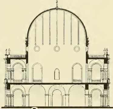
B SECTION
