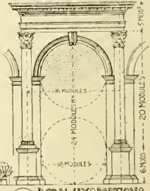
F DOORWAY & PORTION OF COLONNADE WITH PEDESTALS.
