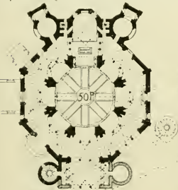
(C) PLAN
