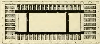
(E) PLAN OF EXISTING LACUNARIA
