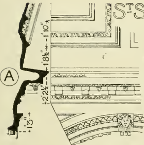
DETAILS OF LOWER PORTION OF DOME
