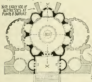
(A) PLAN A DECAGON SUPPORTING A CIRCULAR DOME WITH EARLY FORM OF PENDENTIVES.
